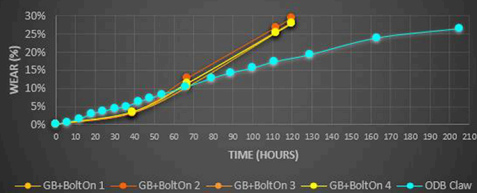
GUTTER STRIPPING BROOM WEAR ODB CLAW™ vs Standard Broom w/Bolt-on Cable
